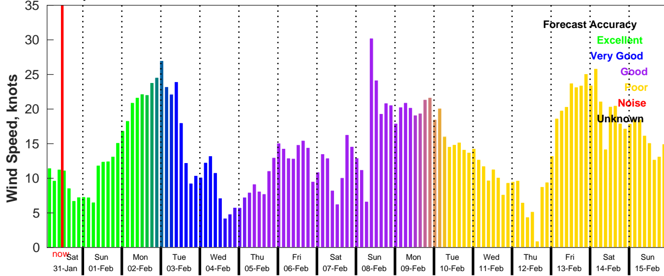
GFS Wind Speed Forecast for NDBC 51000 from 31-Jan-2026 02:00:00 to 16-Feb-2026 02:00:00
