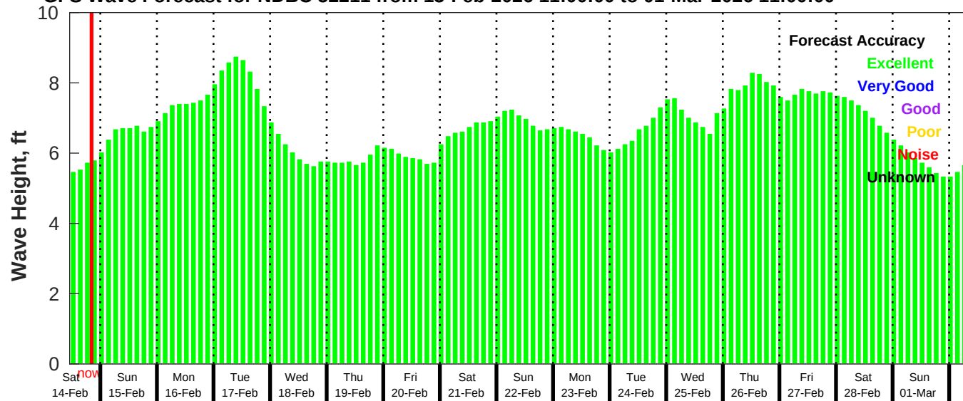
GFS Wave Forecast for NDBC 52211 from 13-Feb-2026 11:00:00 to 01-Mar-2026 11:00:00
