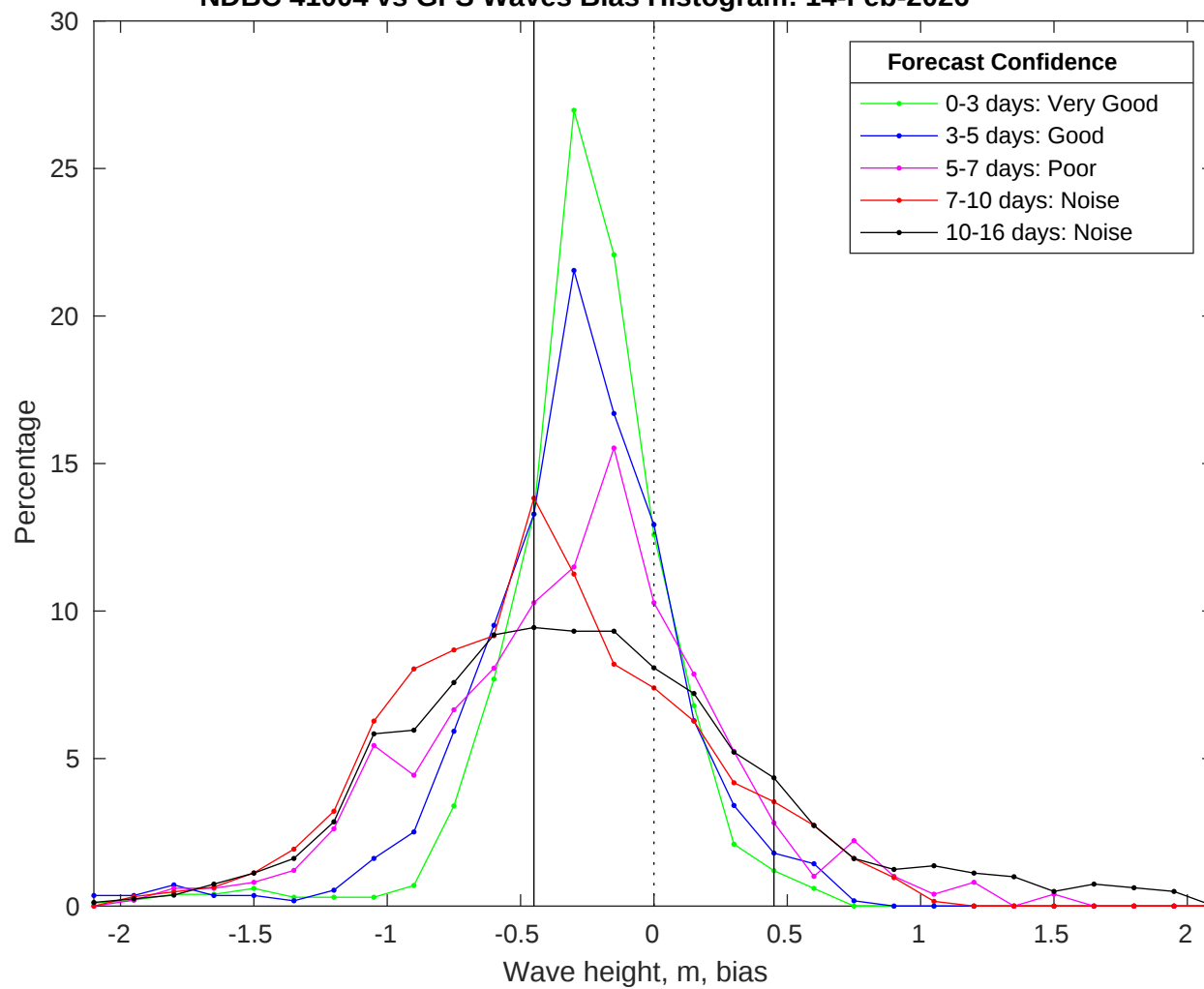
NDBC 41004 vs GFS Waves Bias Histogram: 14-Feb-2026
