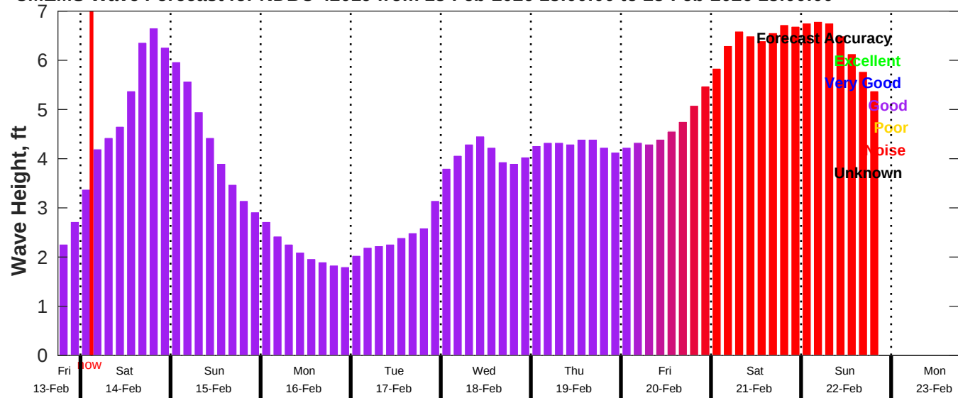
CMEMS Wave Forecast for NDBC 42019 from 13-Feb-2026 18:00:00 to 23-Feb-2026 18:00:00
