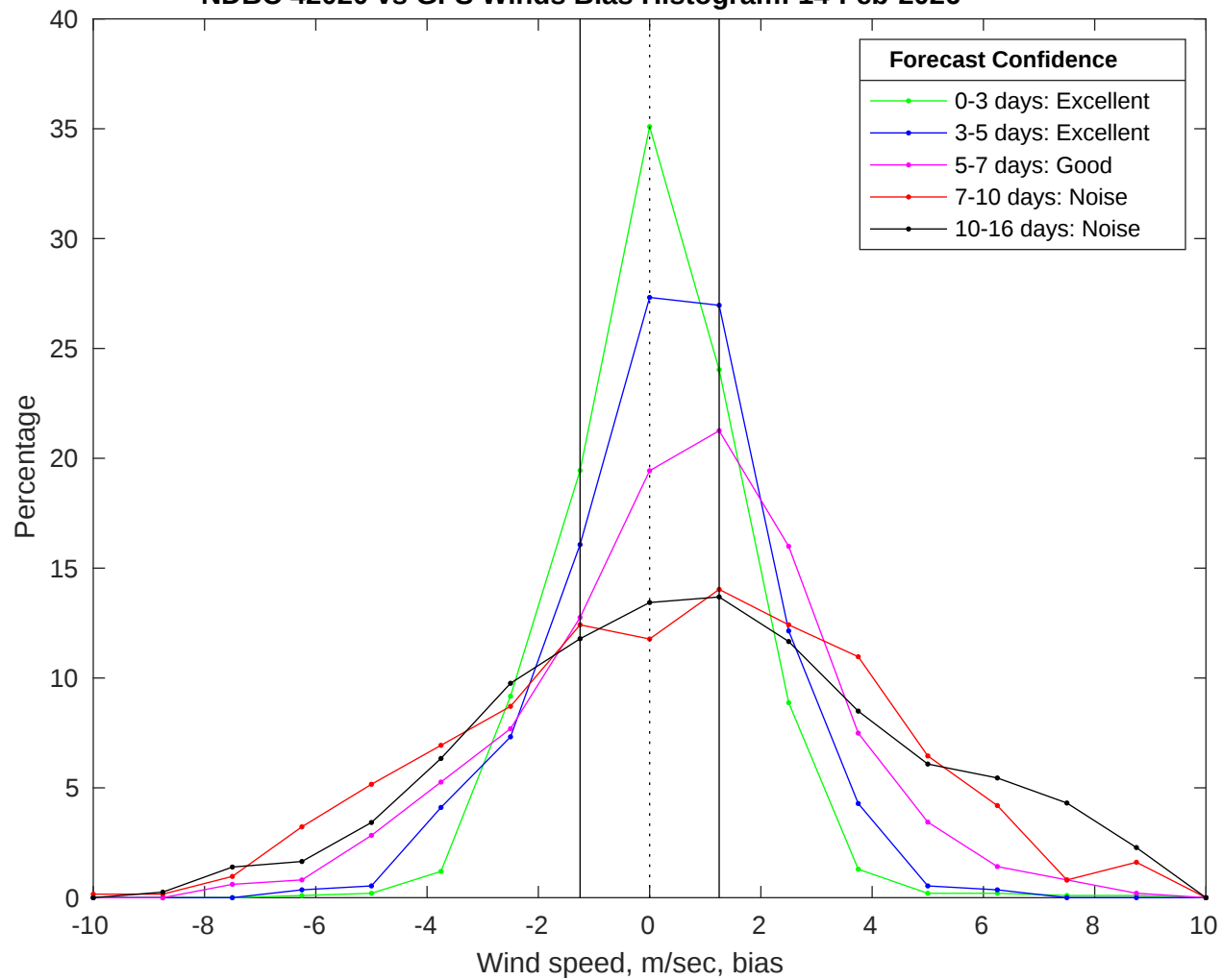
NDBC 42020 vs GFS Winds Bias Histogram: 14-Feb-2026
