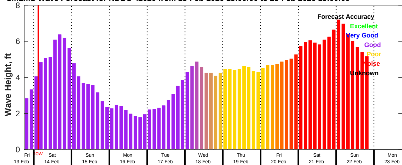
CMEMS Wave Forecast for NDBC 42020 from 13-Feb-2026 18:00:00 to 23-Feb-2026 18:00:00
