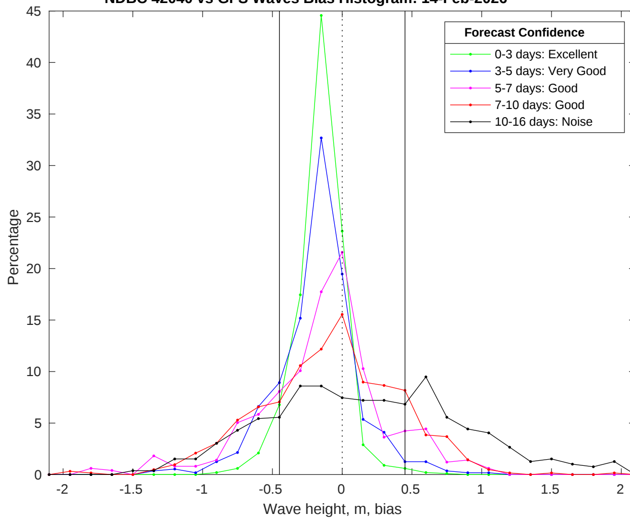
NDBC 42040 vs GFS Waves Bias Histogram: 14-Feb-2026
