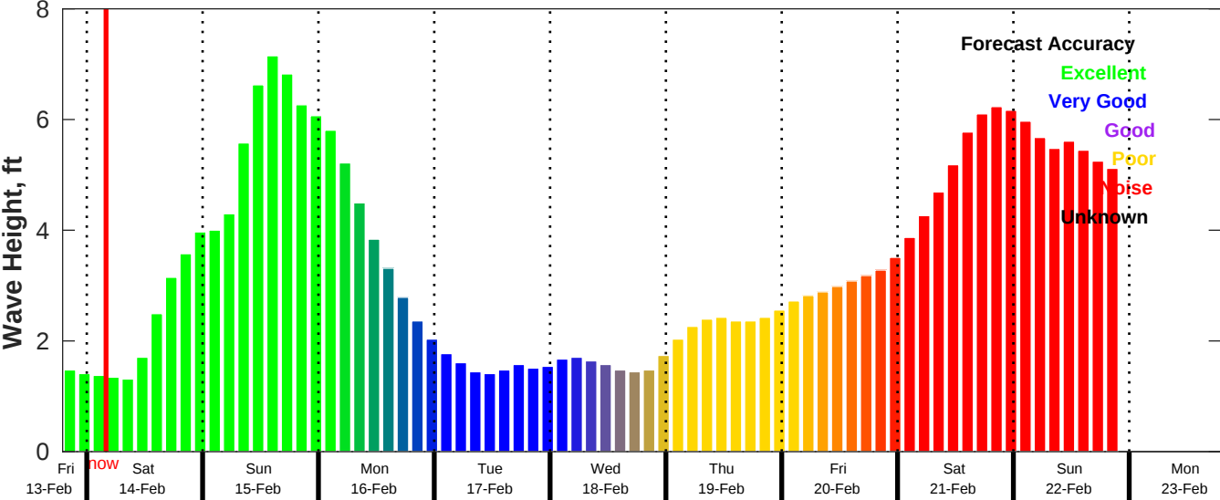
CMEMS Wave Forecast for NDBC 42040 from 13-Feb-2026 19:00:00 to 23-Feb-2026 19:00:00
