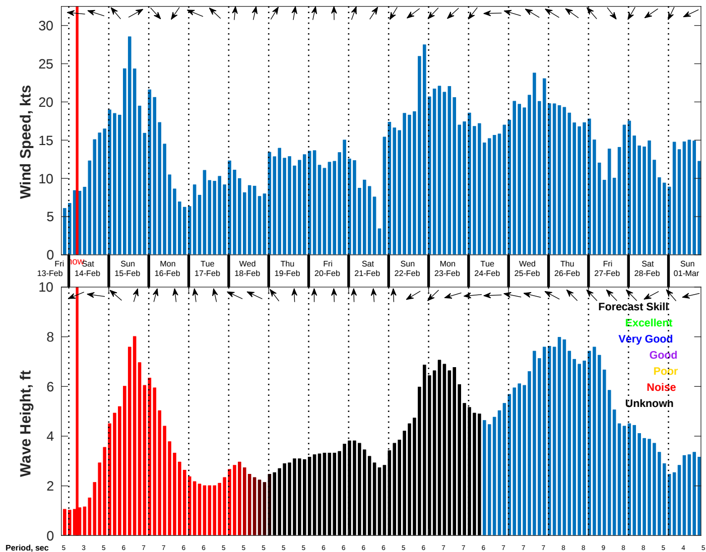
Wind & Wave Forecast for NDBC 42058 from 13-Feb-2026 20:00:00 to 01-Mar-2026 20:00:00
