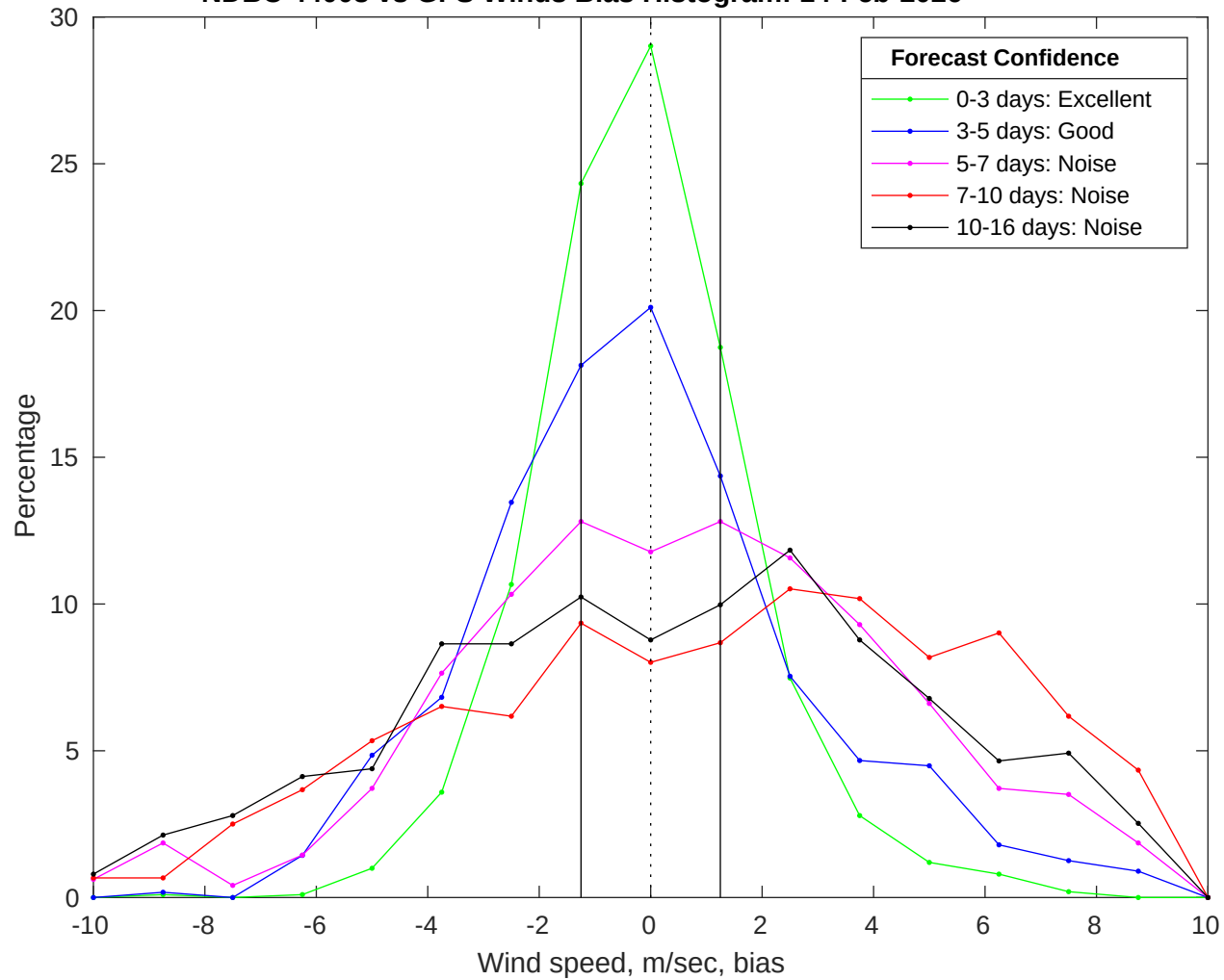
NDBC 44008 vs GFS Winds Bias Histogram: 14-Feb-2026
