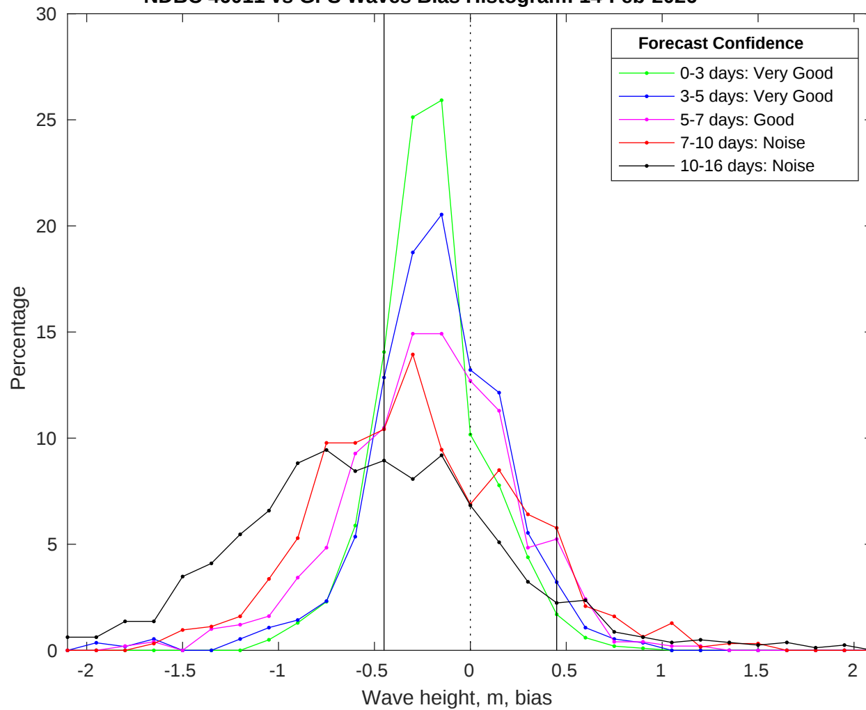
NDBC 46011 vs GFS Waves Bias Histogram: 14-Feb-2026
