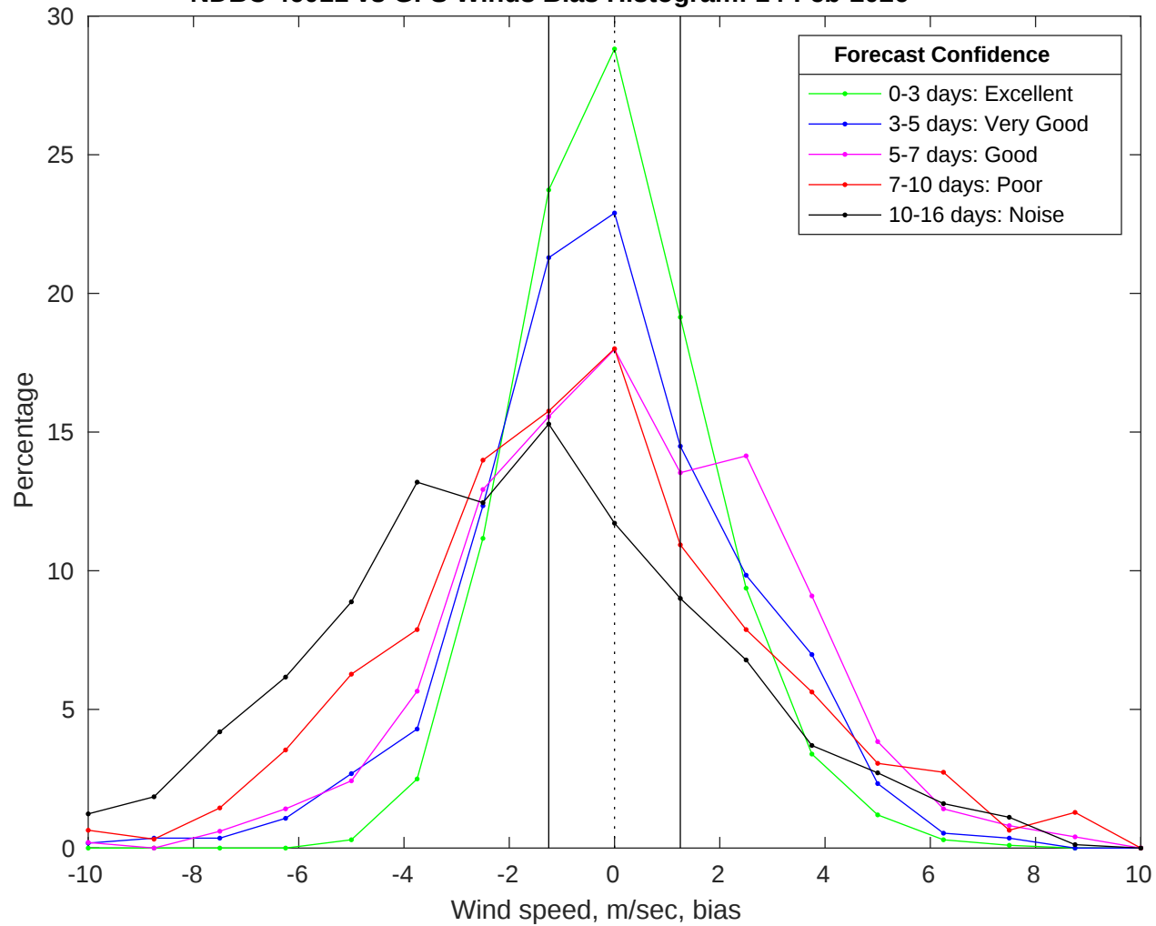
NDBC 46011 vs GFS Winds Bias Histogram: 14-Feb-2026
