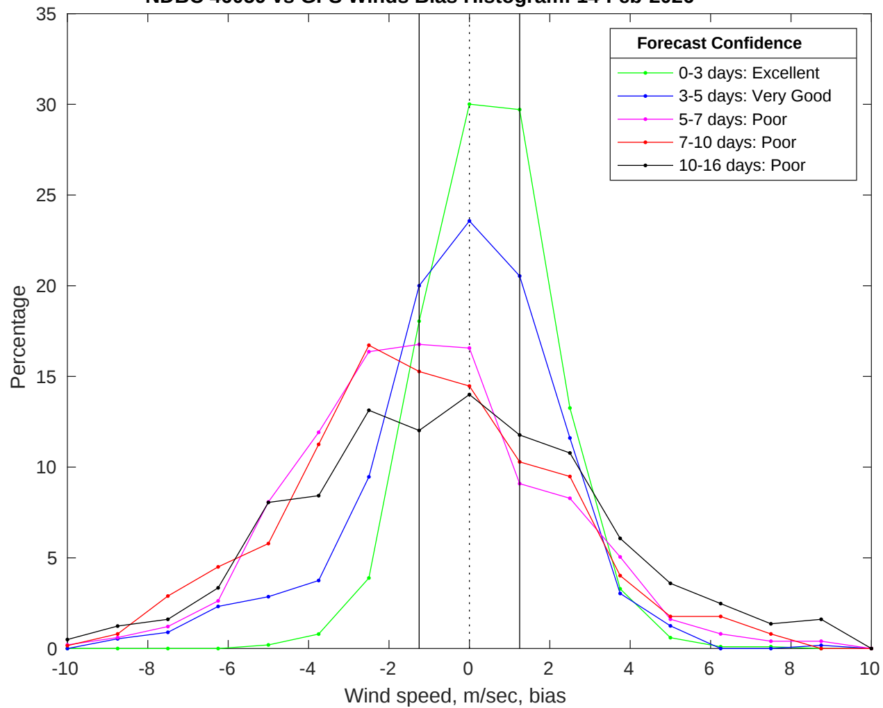
NDBC 46059 vs GFS Winds Bias Histogram: 14-Feb-2026
