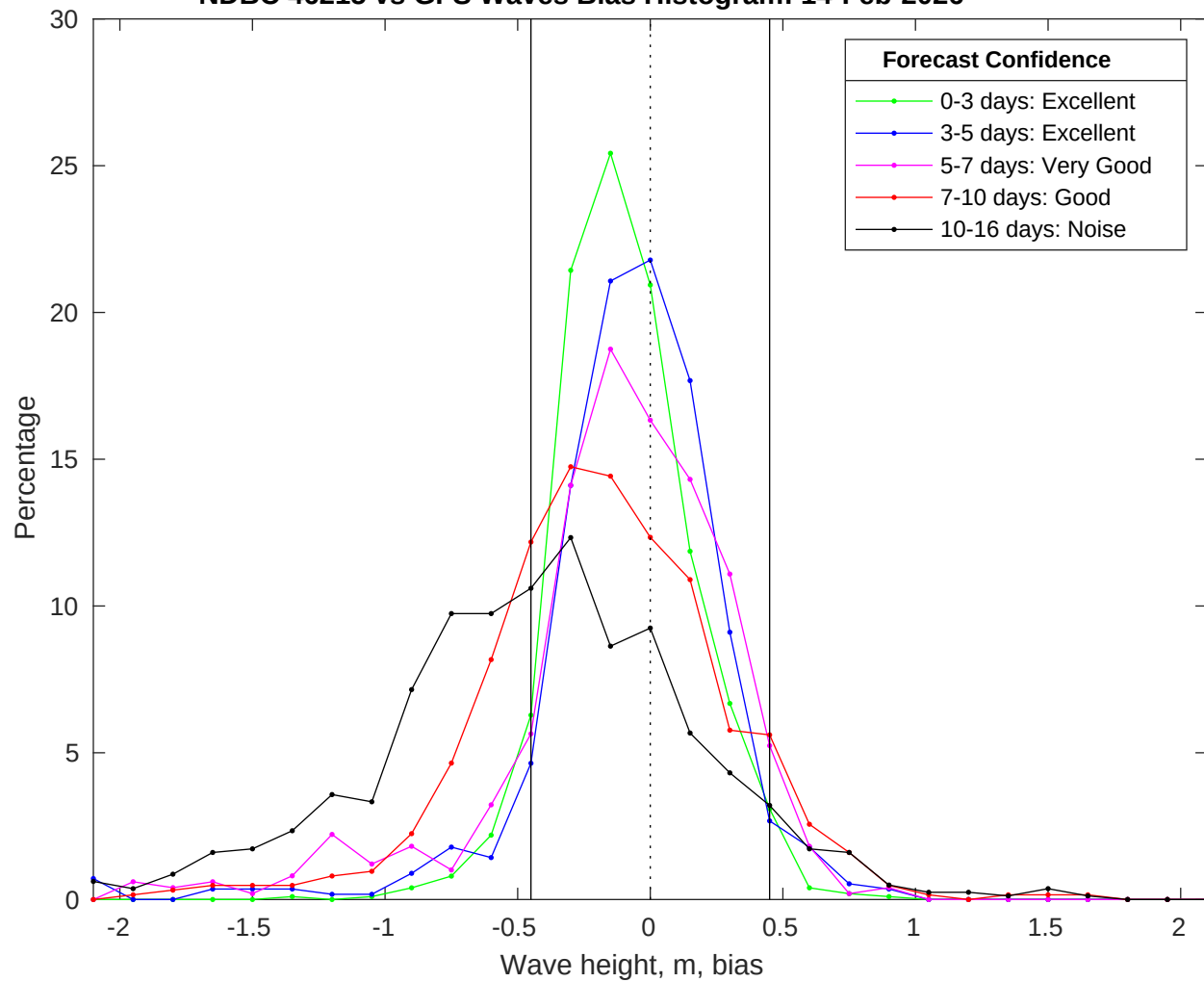
NDBC 46215 vs GFS Waves Bias Histogram: 14-Feb-2026
