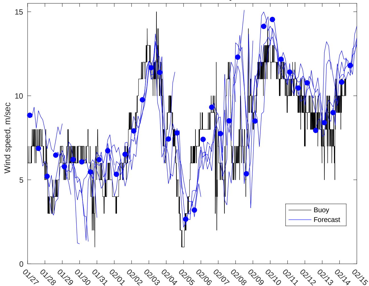
NDBC 51000 vs GFS Winds: 3 to 5 day forecast
