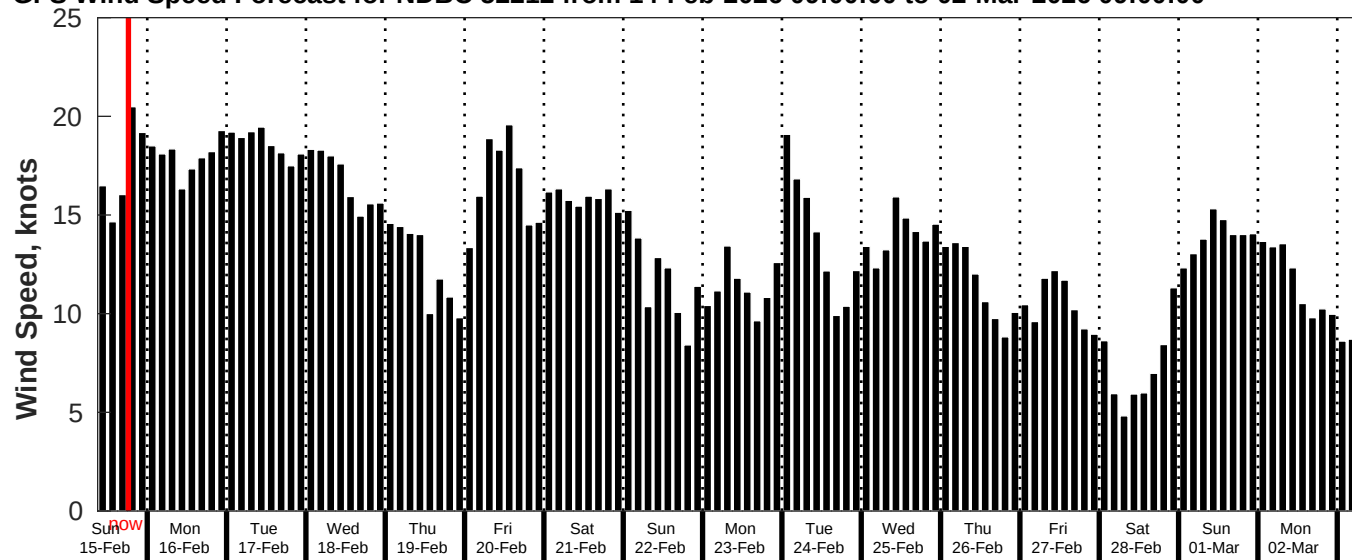
GFS Wind Speed Forecast for NDBC 52212 from 14-Feb-2026 09:00:00 to 02-Mar-2026 09:00:00
