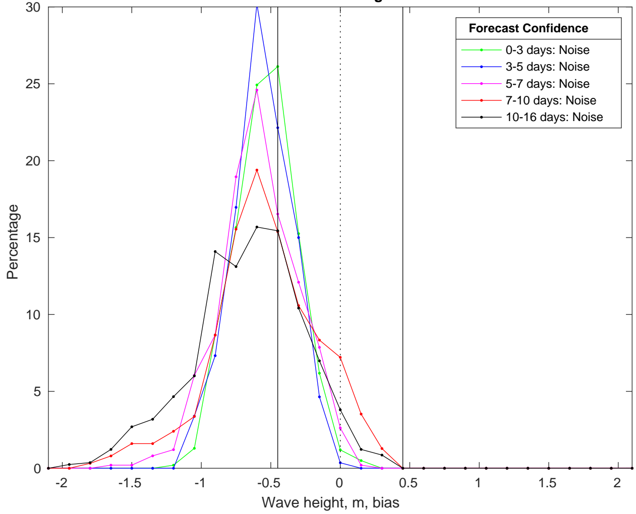
NDBC 52213 vs GFS Waves Bias Histogram: 14-Feb-2026
