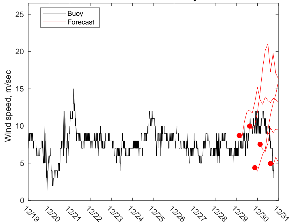
NDBC 41002 vs GFSWinds: 10 to 16 day forecast
