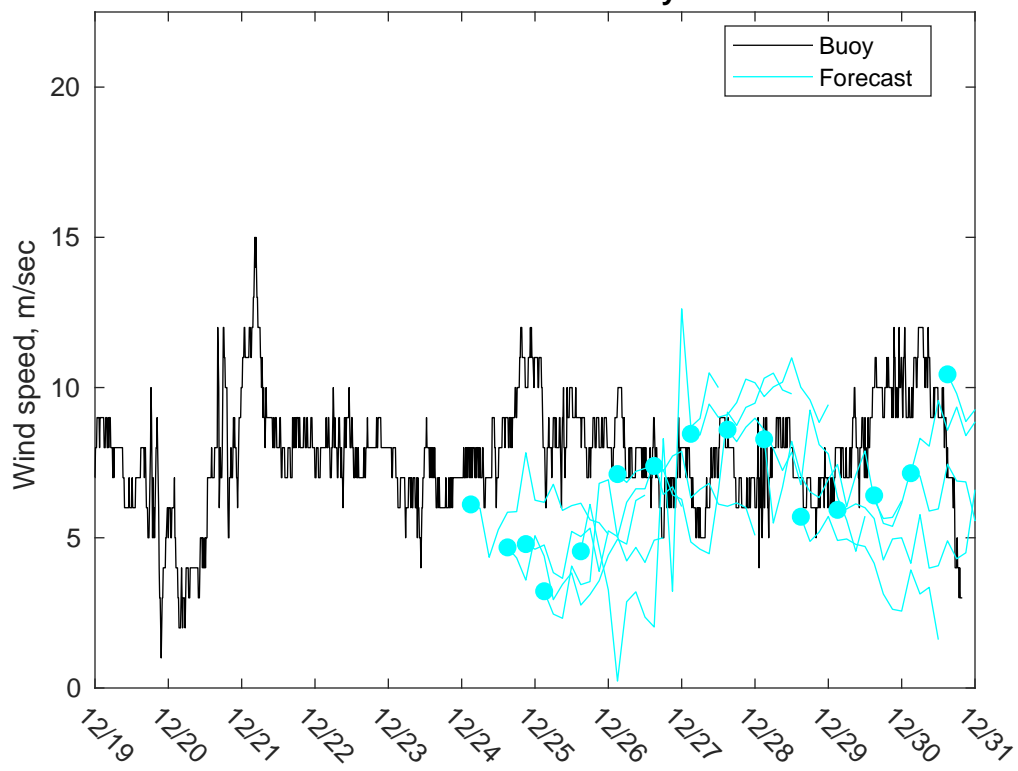
NDBC 41002 vs GFSWinds: 5 to 7 day forecast
