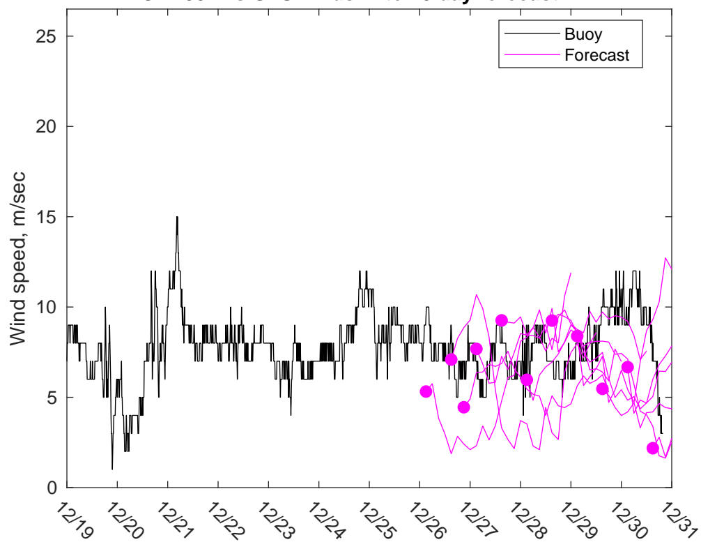
NDBC 41002 vs GFSWinds: 7 to 10 day forecast
