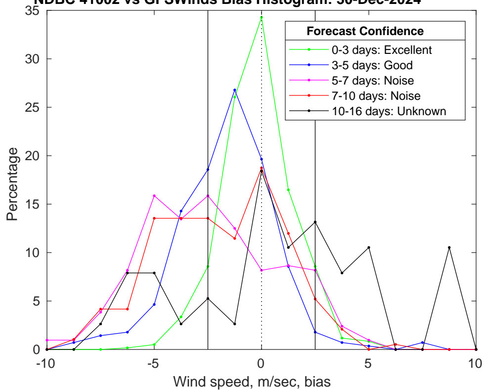
NDBC 41002 vs GFSWinds Bias Histogram: 30-Dec-2024
