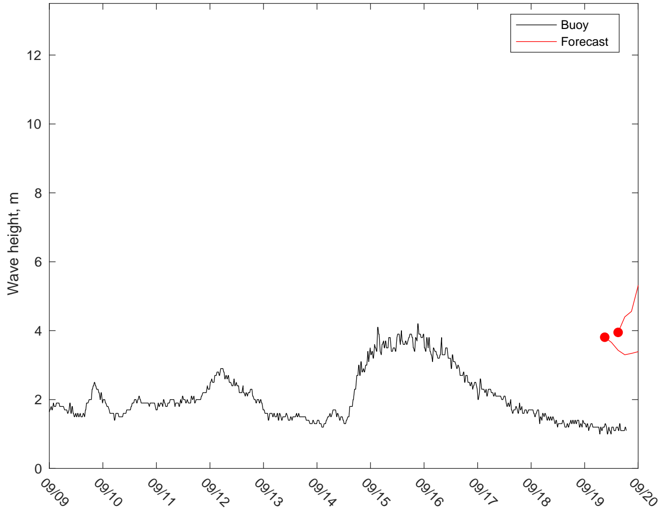
NDBC 41002 vs GFSWaves: 10 to 16 day forecast
