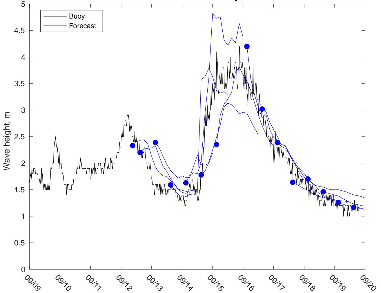
NDBC 41002 vs GFSWaves: 3 to 5 day forecast
