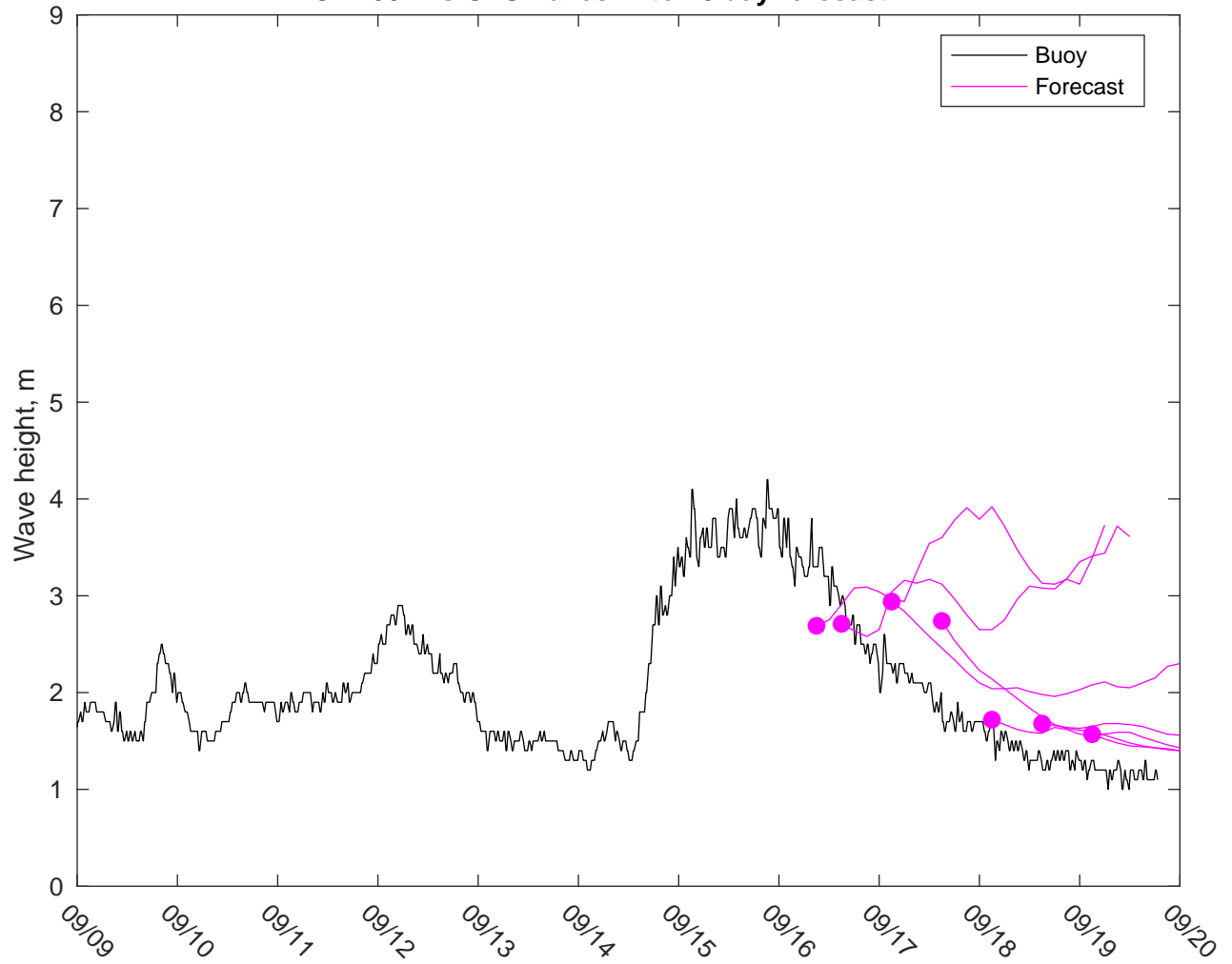
NDBC 41002 vs GFSWaves: 7 to 10 day forecast
