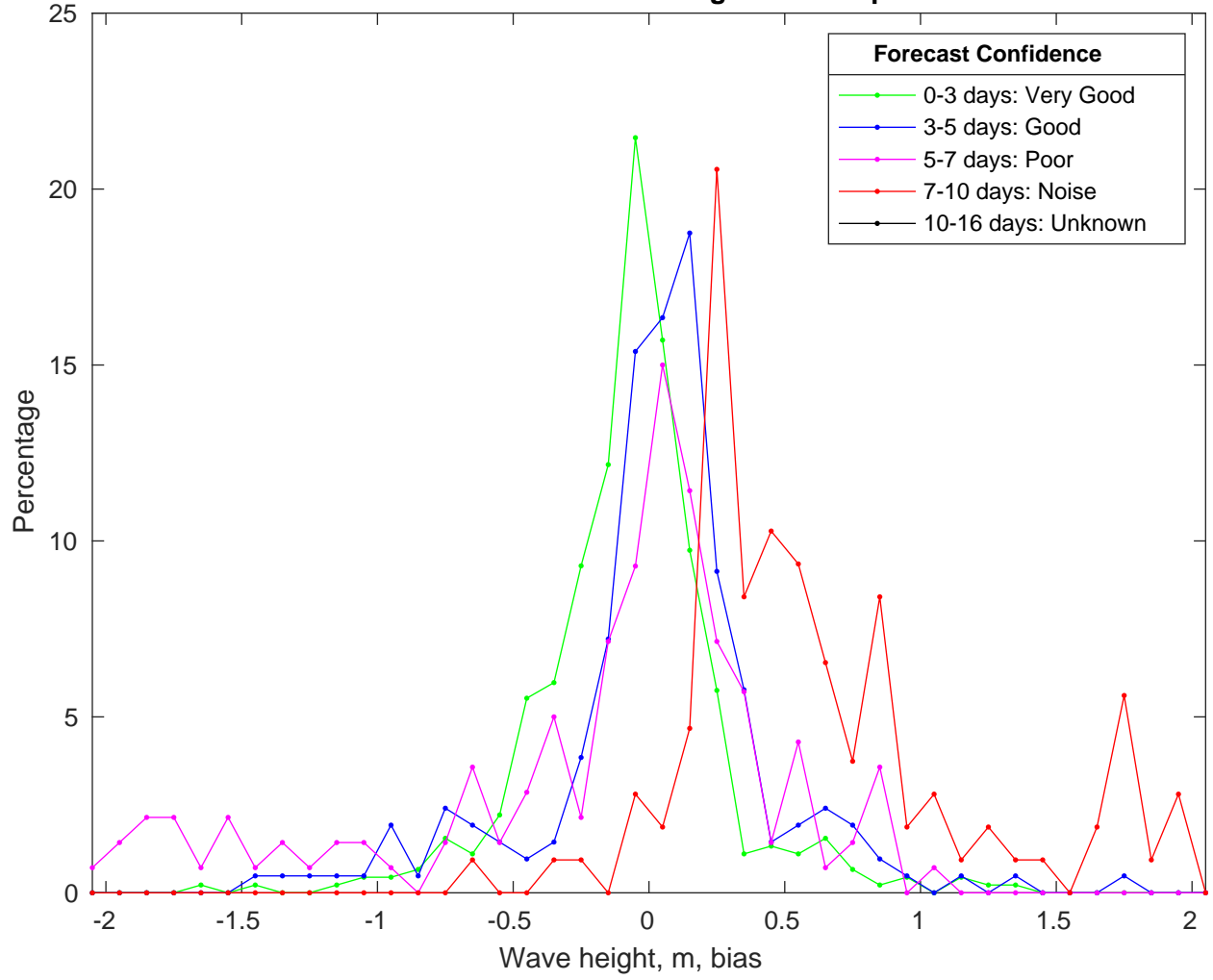
NDBC 41002 vs GFSWaves Bias Histogram: 19-Sep-2024
