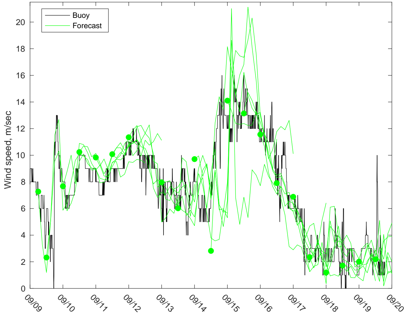
NDBC 41002 vs GFSWinds: 0 to 3 day forecast
