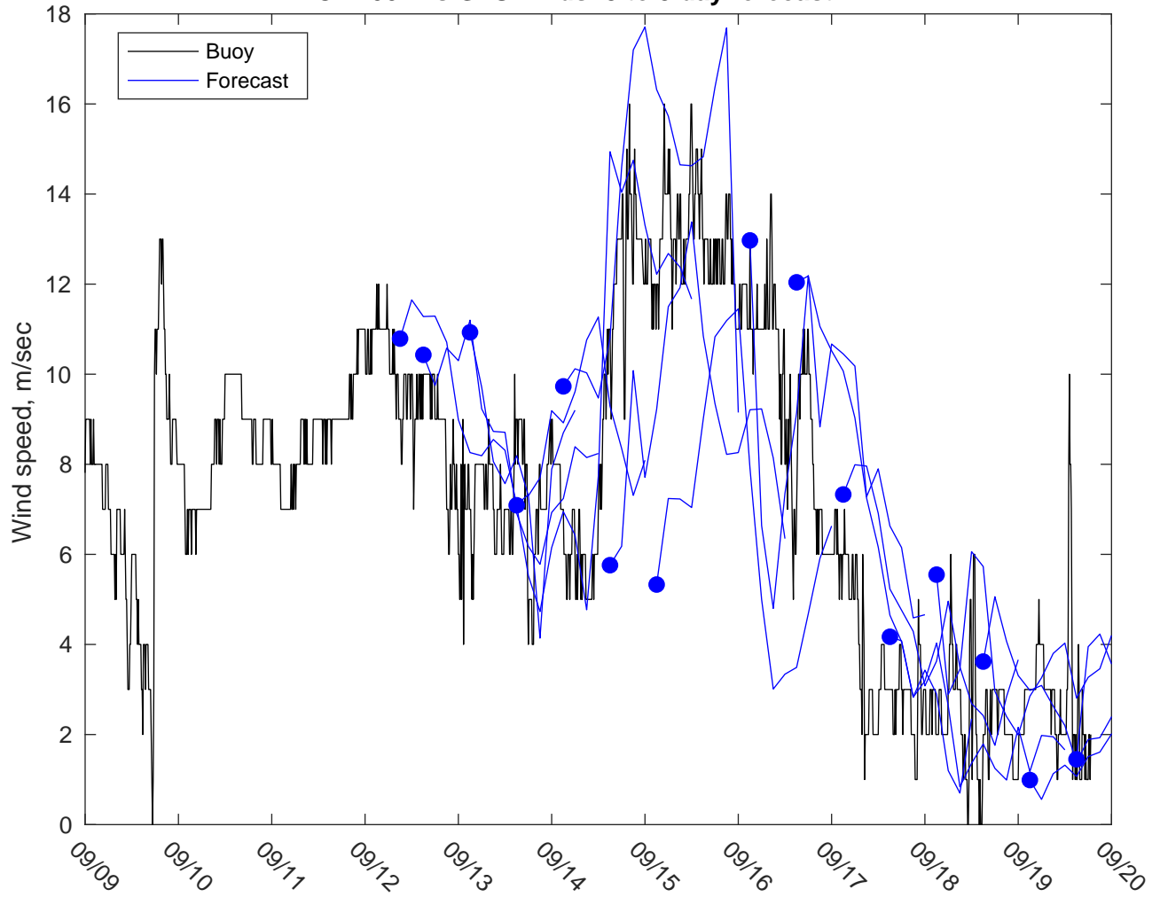
NDBC 41002 vs GFSWinds: 3 to 5 day forecast
