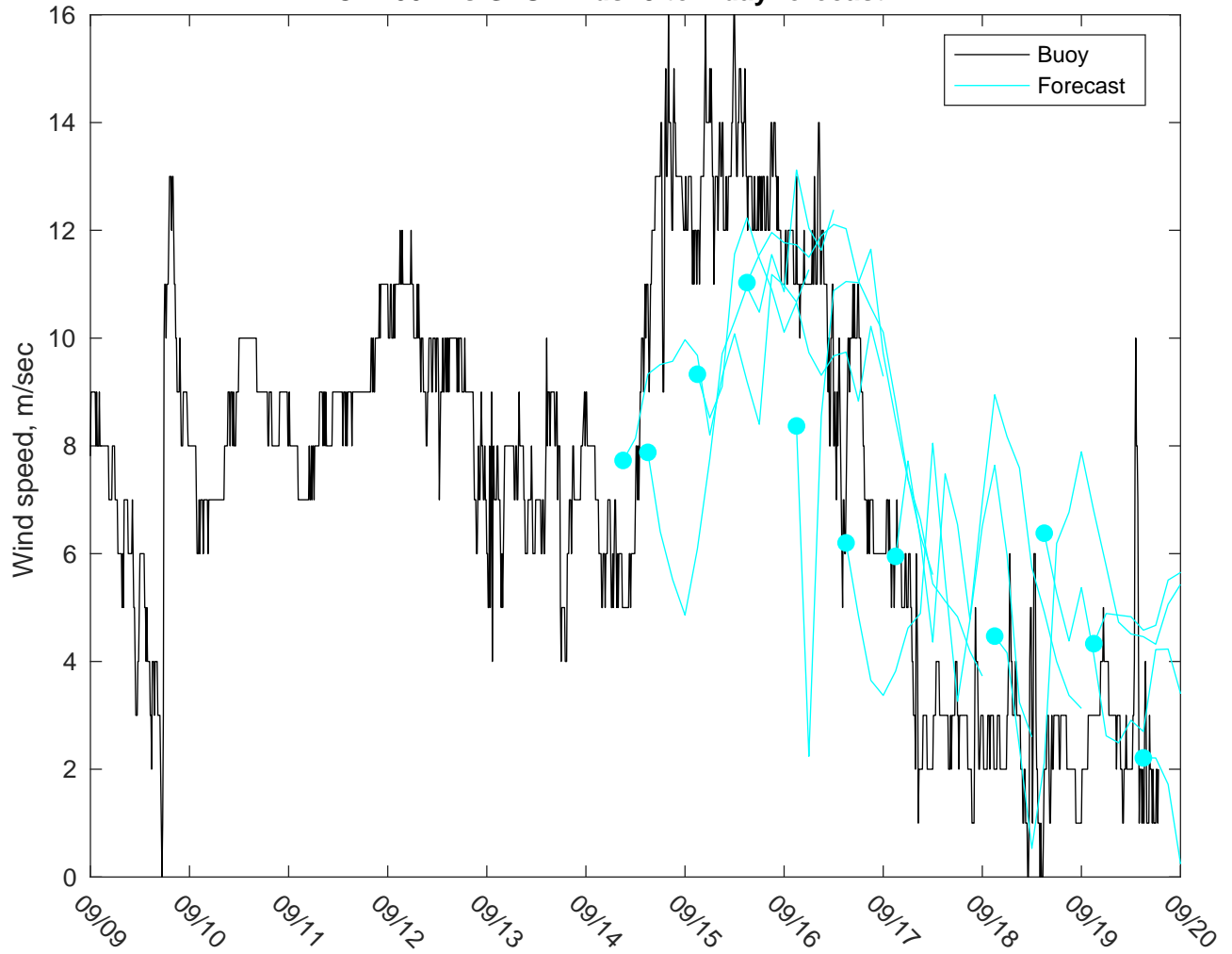
NDBC 41002 vs GFSWinds: 5 to 7 day forecast
