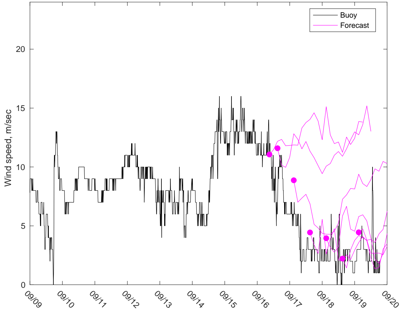
NDBC 41002 vs GFSWinds: 7 to 10 day forecast
