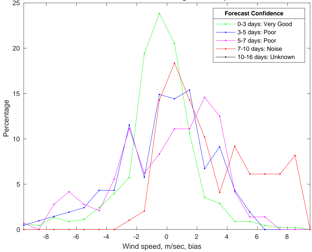
NDBC 41002 vs GFS Winds Bias Histogram: 19-Sep-2024
