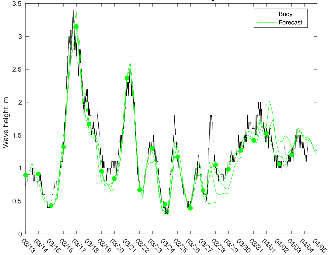
NDBC 41004 vs AUSWAV Waves: 0 to 3 day forecast
