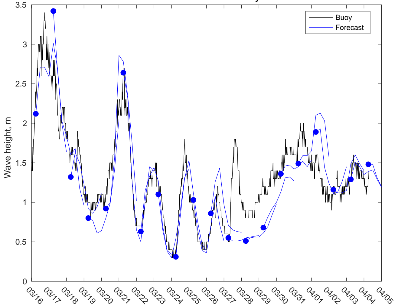
NDBC 41004 vs AUSWAV Waves: 3 to 5 day forecast
