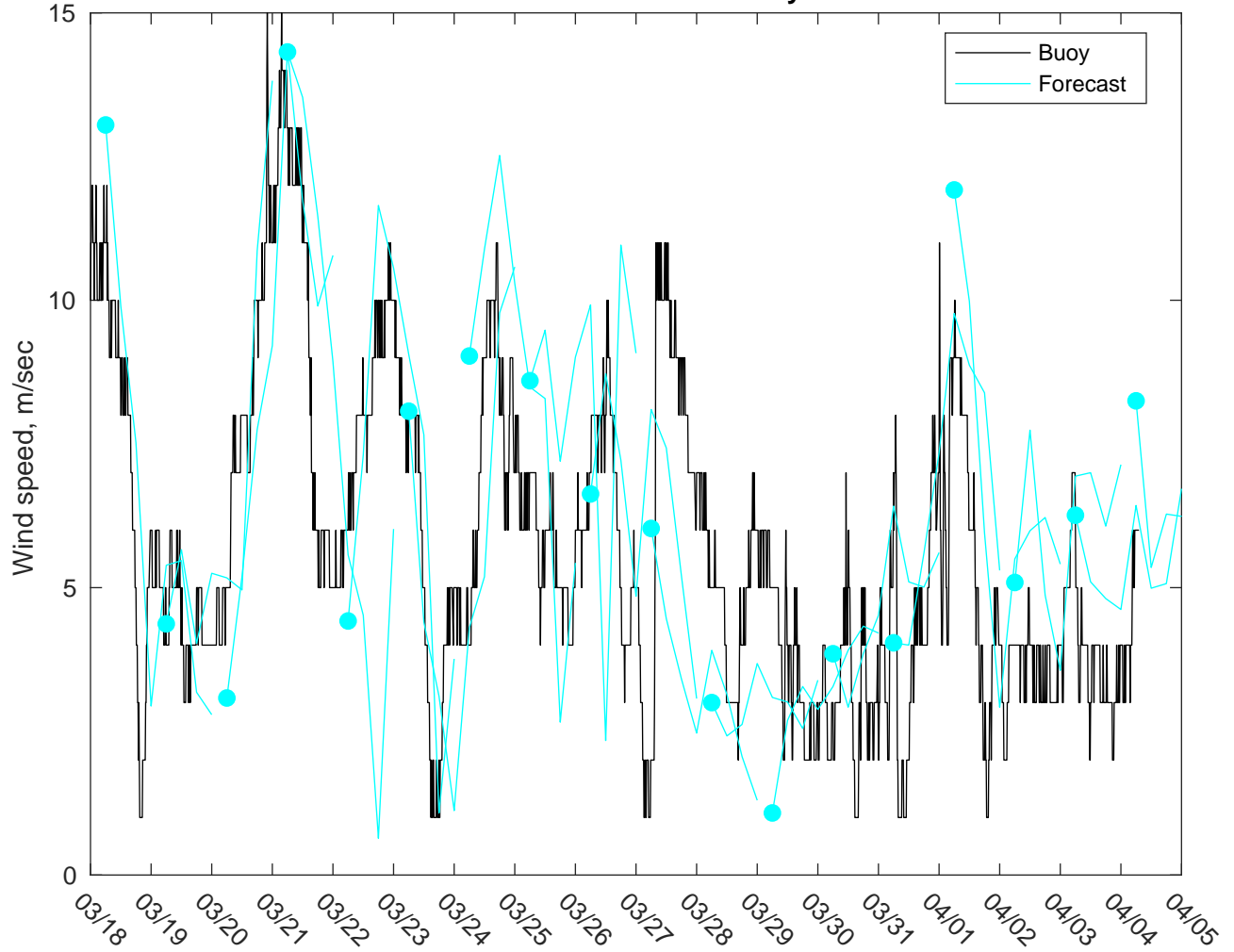
NDBC 41004 vs AUSWAV Winds: 5 to 7 day forecast
