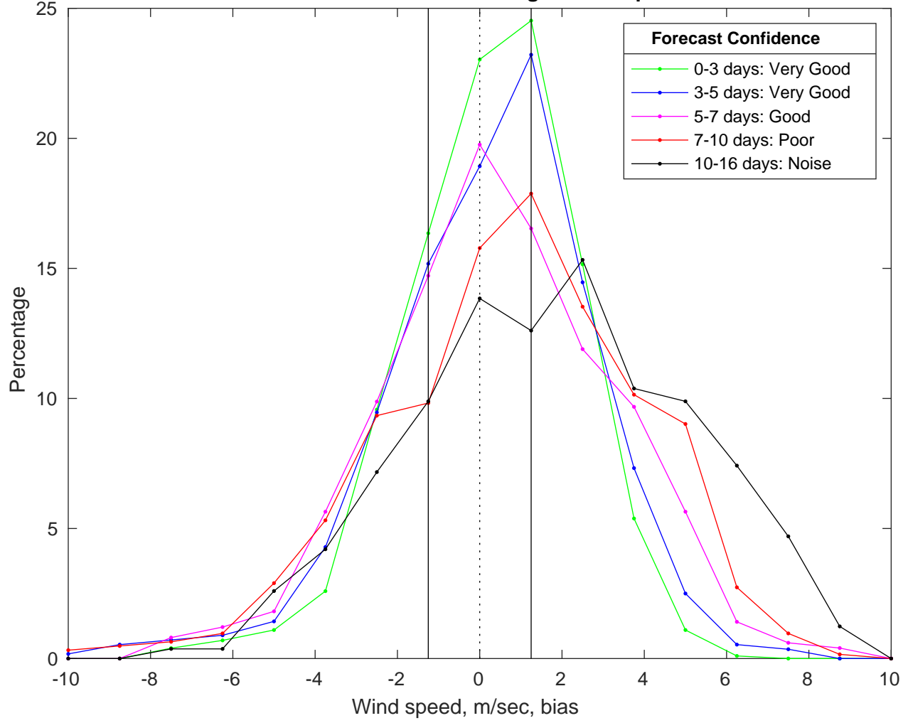
NDBC 41004 vs GFS Winds Bias Histogram: 04-Apr-2025
