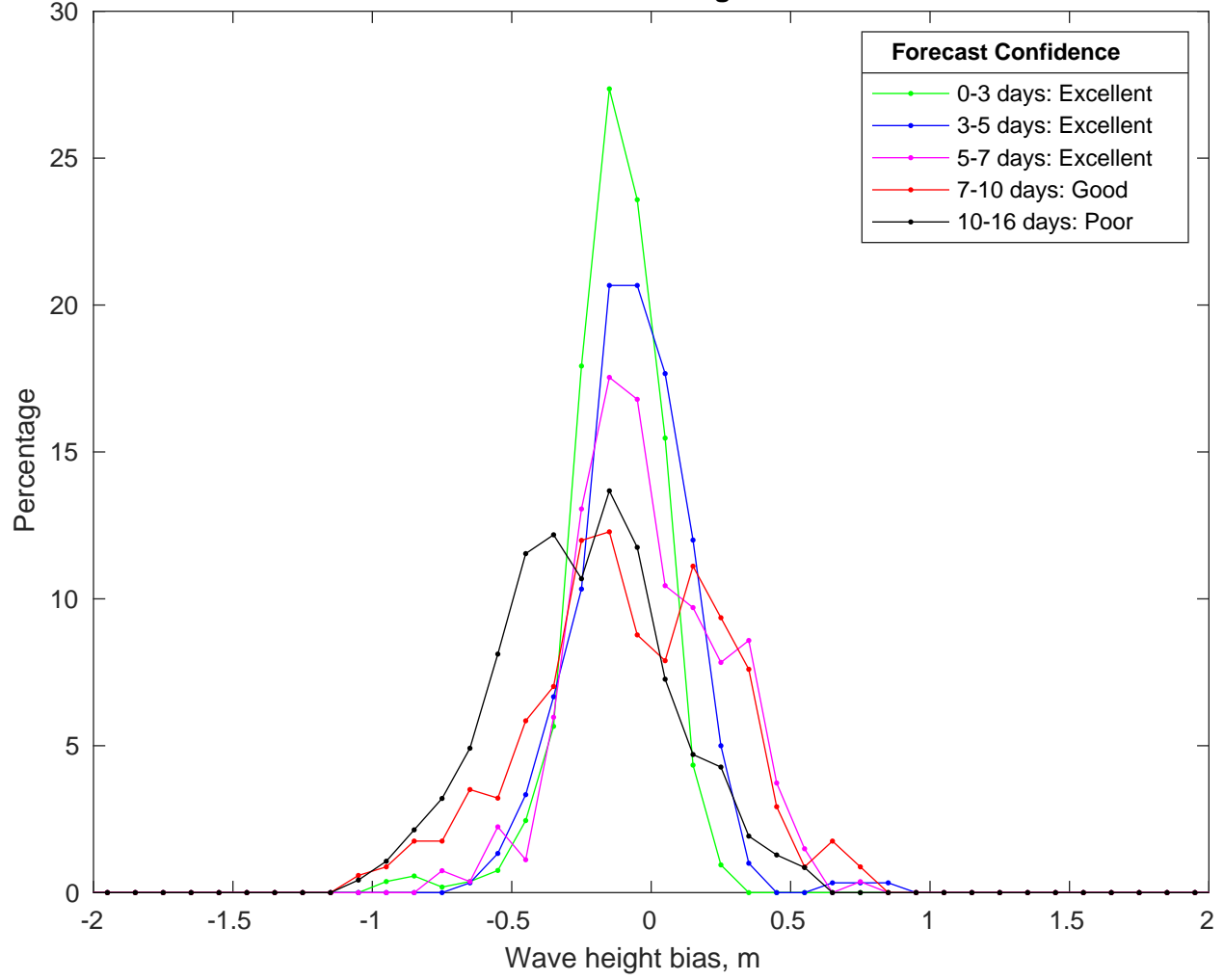
NDBC 41004 vs GFSWave Bias Histogram: 20-Jul-2024
