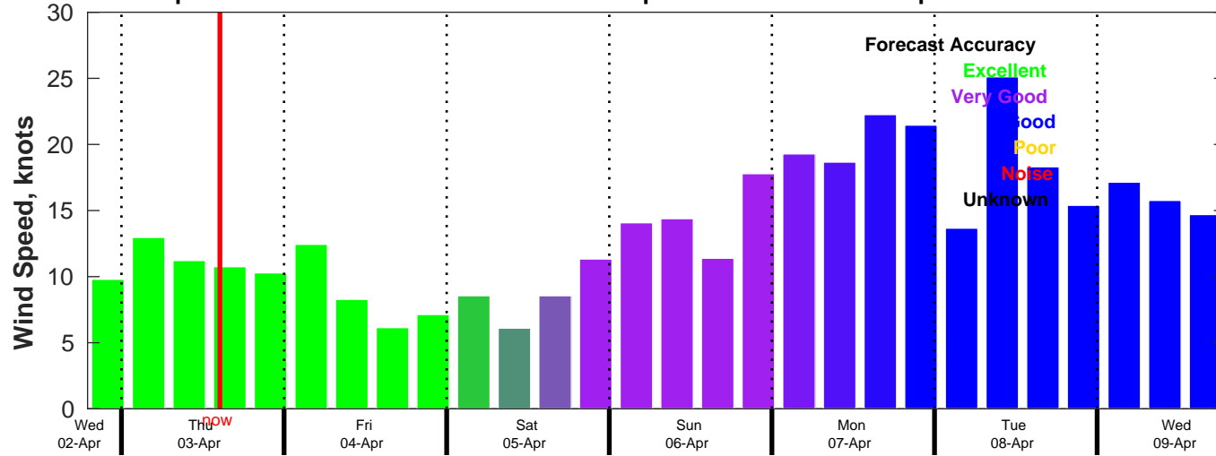
AUSWAV Wind Speed Forecast for NDBC 41004 from 02-Apr-2025 19:00:00 to 09-Apr-2025 19:00:00
