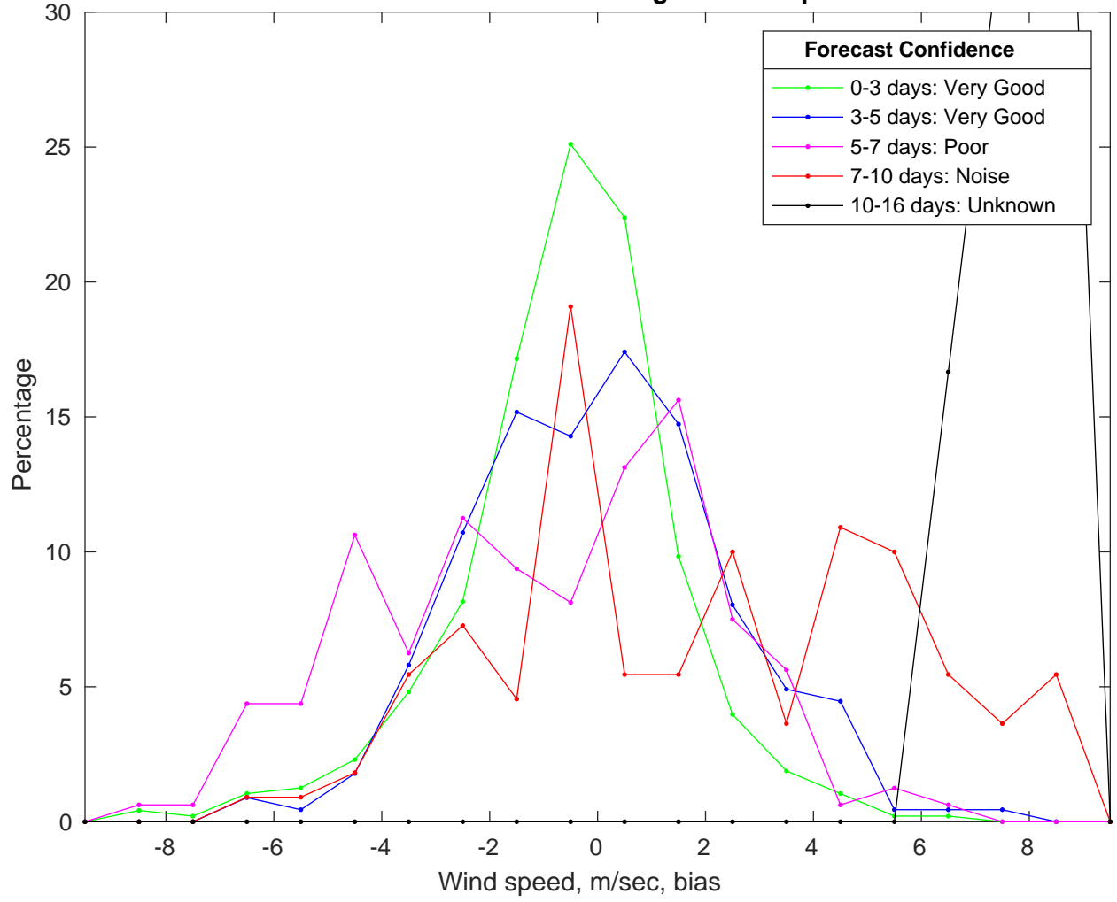
NDBC 41004 vs GFSWinds Bias Histogram: 19-Sep-2024
