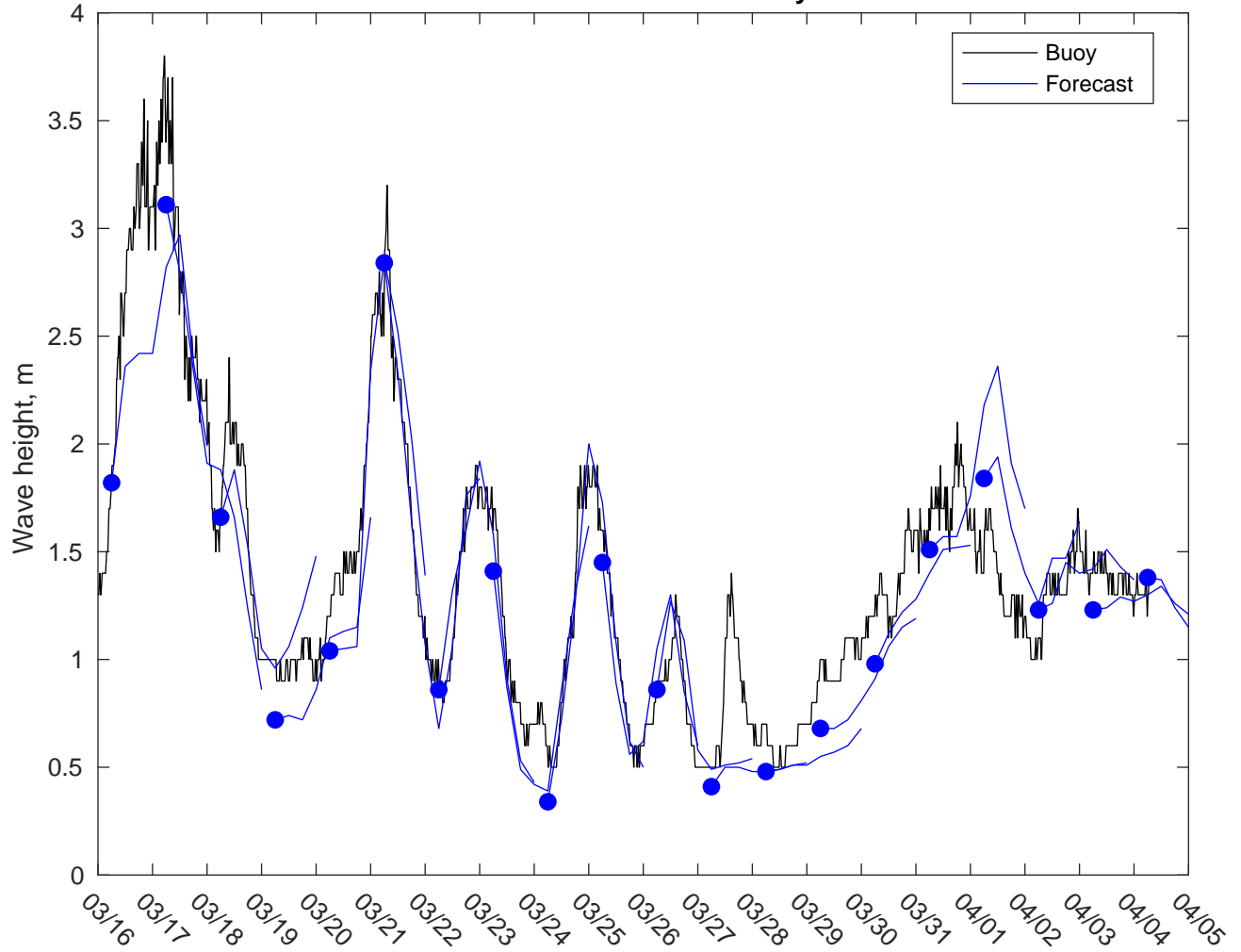
NDBC 41013 vs AUSWAV Waves: 3 to 5 day forecast
