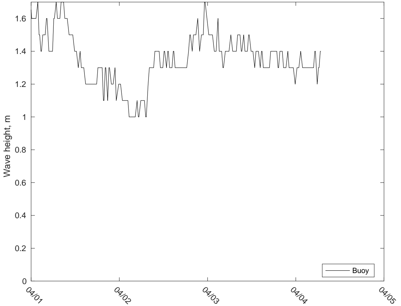
NDBC 41013 vs AUSWAV Waves: 7 to 10 day forecast
