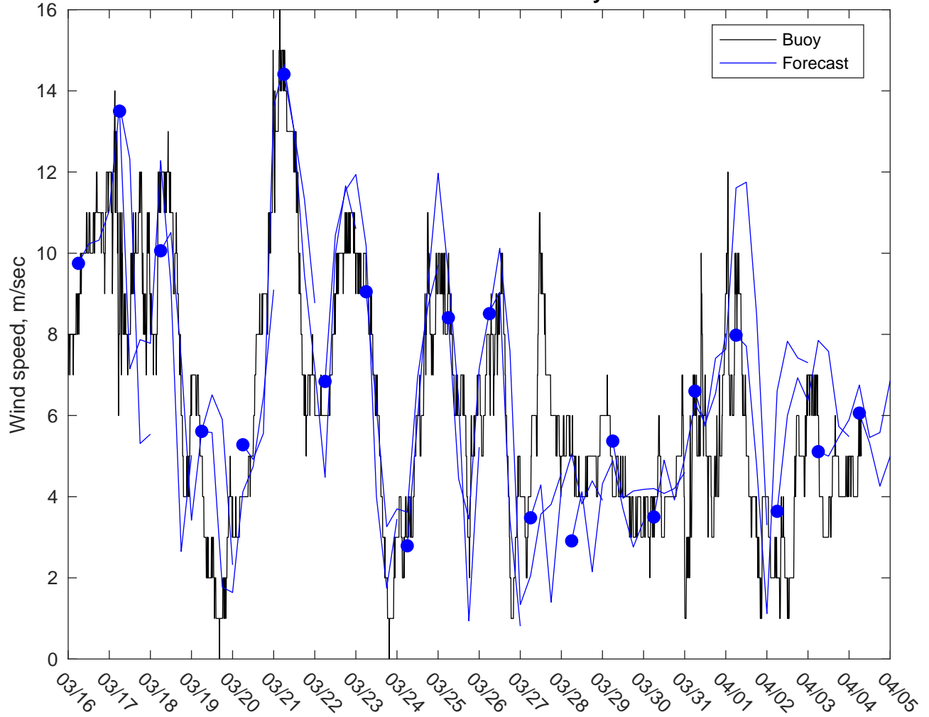
NDBC 41013 vs AUSWAV Winds: 3 to 5 day forecast
