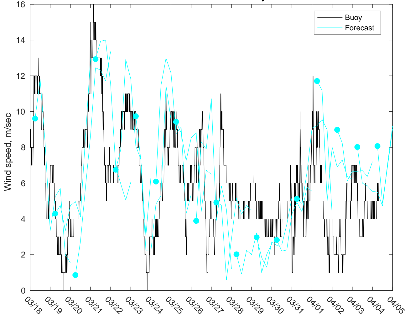
NDBC 41013 vs AUSWAV Winds: 5 to 7 day forecast
