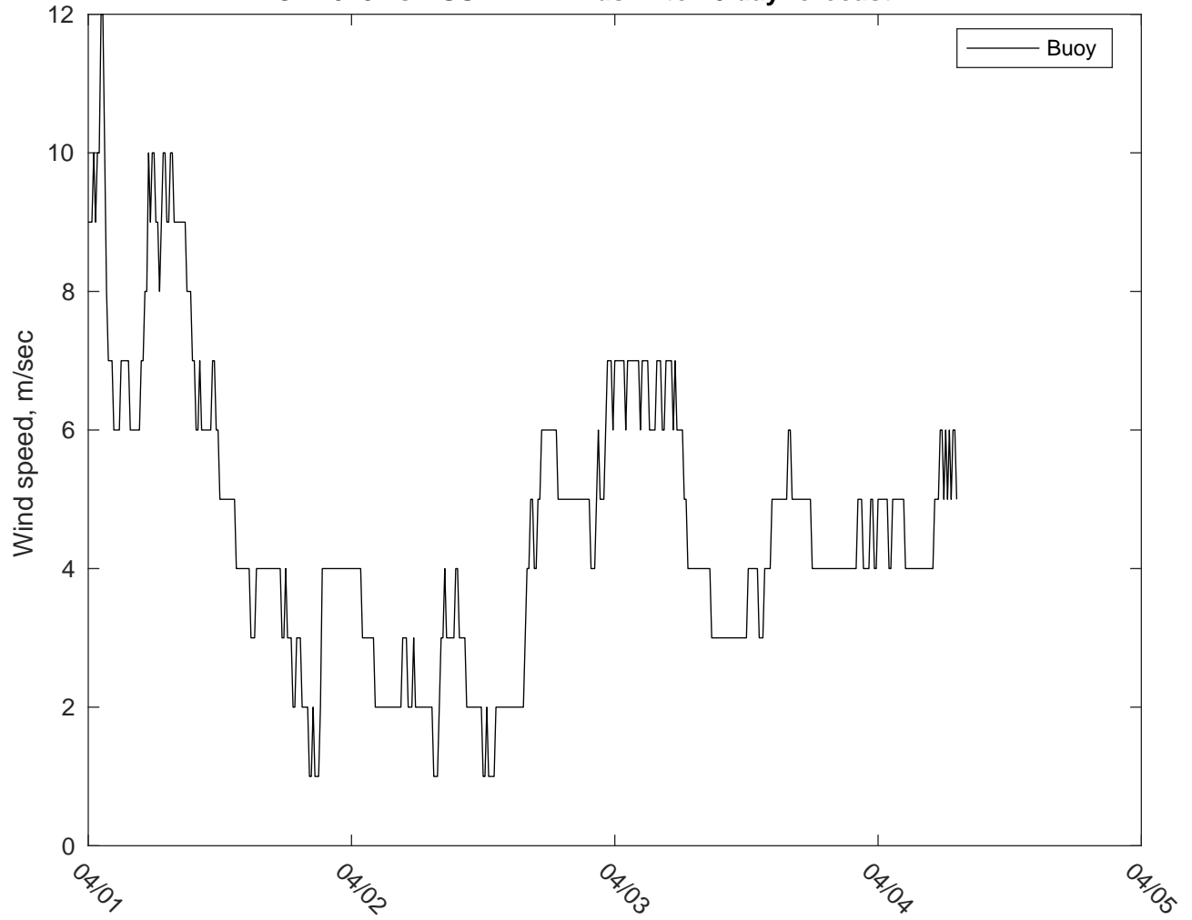
NDBC 41013 vs AUSWAV Winds: 7 to 10 day forecast
