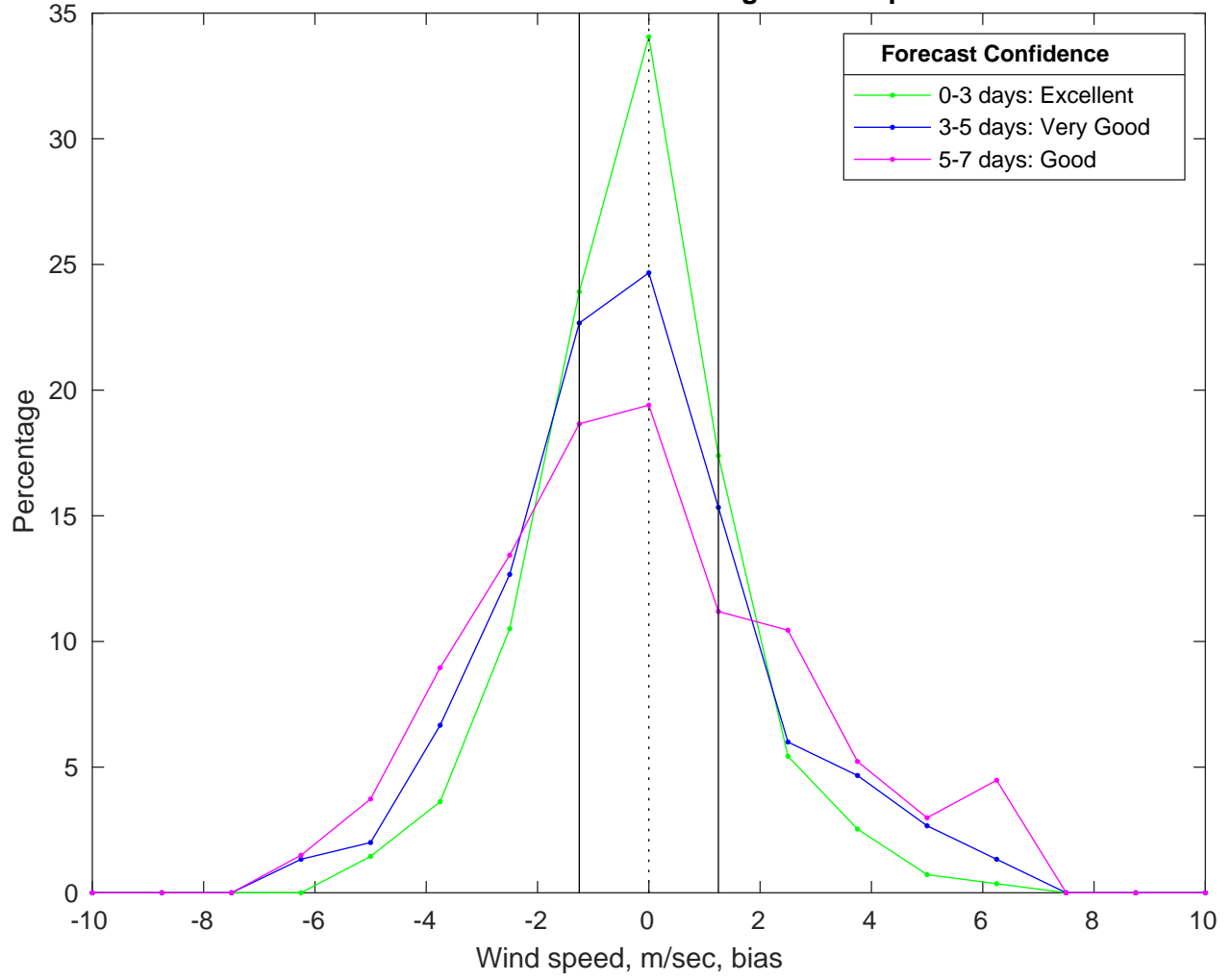
NDBC 41013 vs AUSWAV Winds Bias Histogram: 04-Apr-2025
