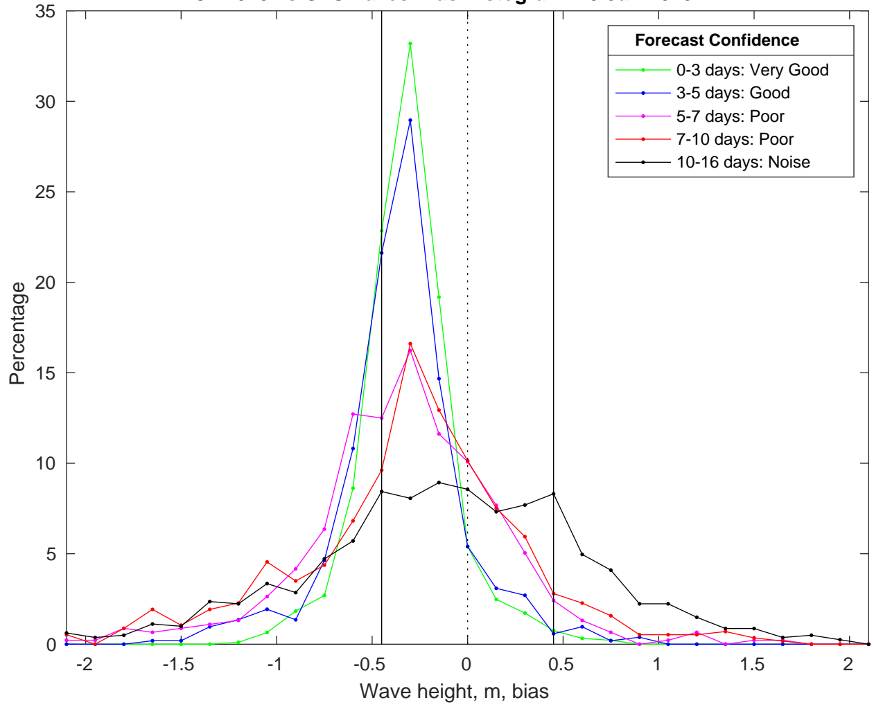
NDBC 41013 vs GFSWaves Bias Histogram: 18-Jan-2025
