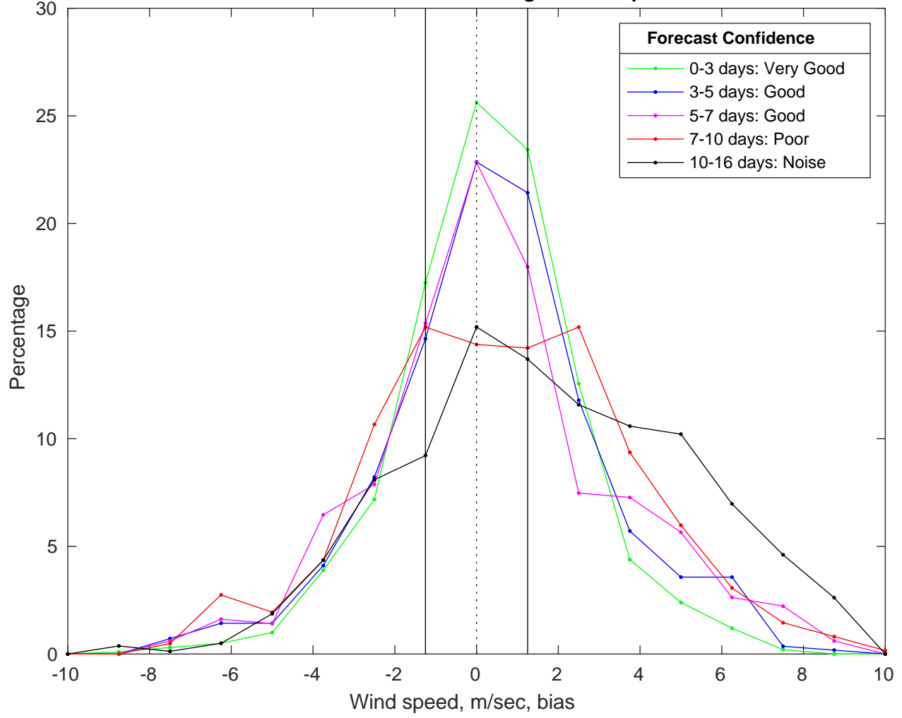
NDBC 41013 vs GFS Winds Bias Histogram: 04-Apr-2025
