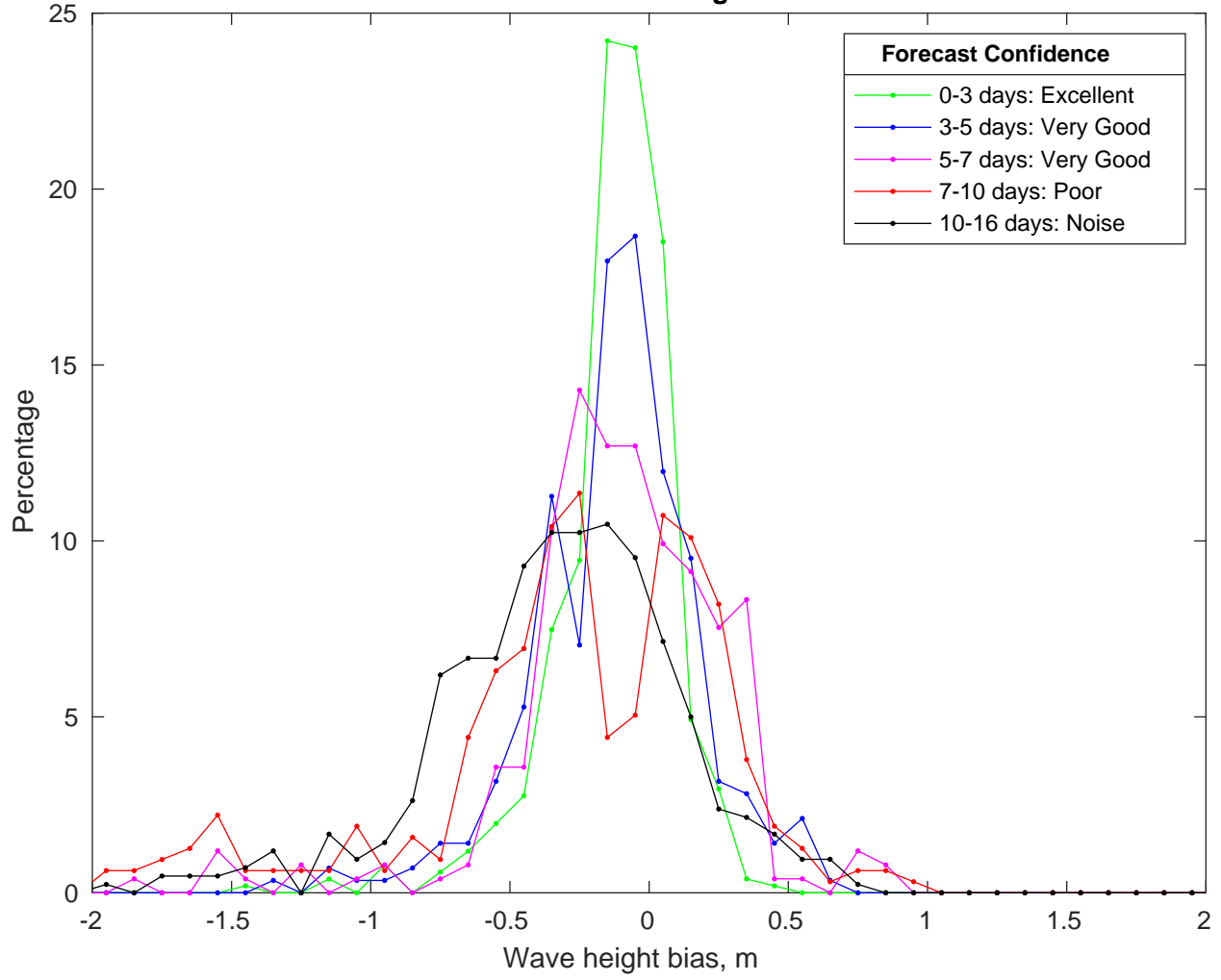
NDBC 41013 vs GFSWave Bias Histogram: 20-Jul-2024
