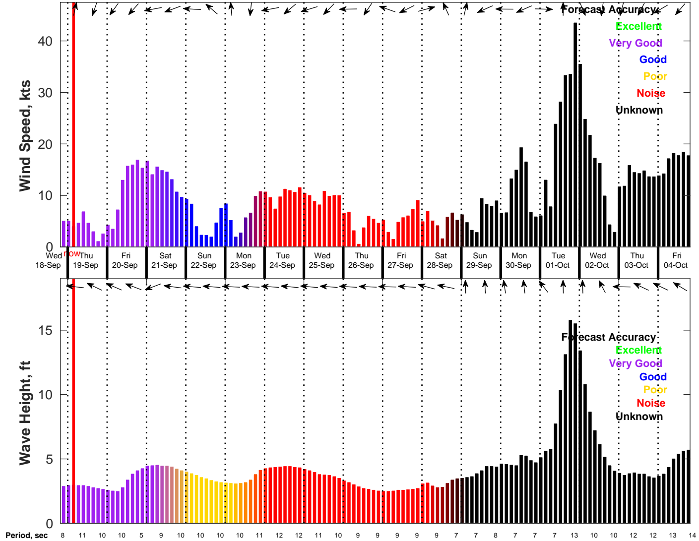
Wind & Wave Forecast for NDBC 41013 from 18-Sep-2024 20:00:00 to 04-Oct-2024 20:00:00
