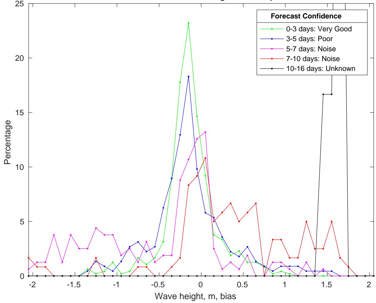
NDBC 41013 vs GFSWaves Bias Histogram: 19-Sep-2024
