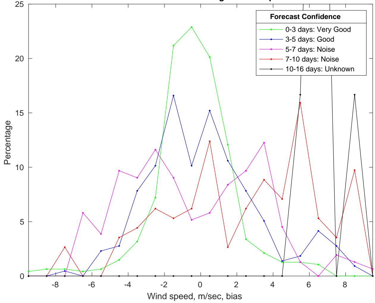
NDBC 41013 vs GFS Winds Bias Histogram: 19-Sep-2024
