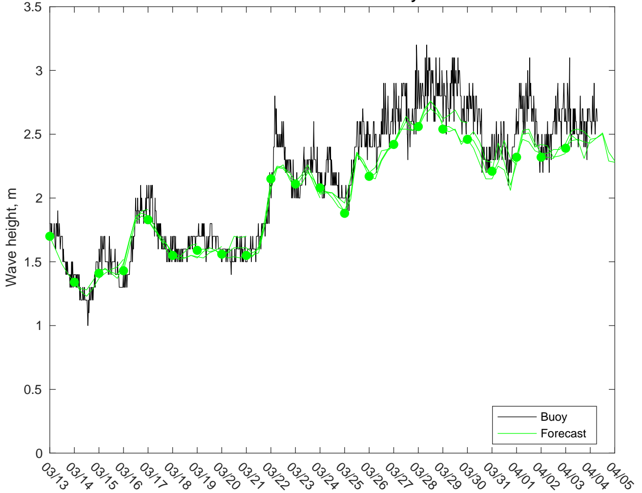
NDBC 41040 vs AUSWAV Waves: 0 to 3 day forecast
